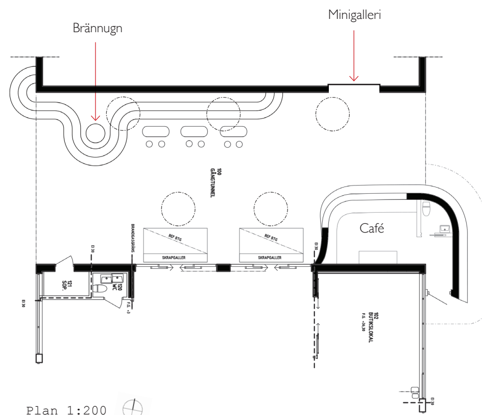
Plan 1:200
